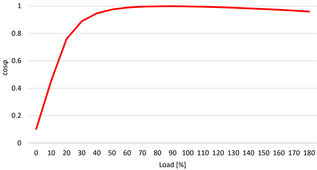
Figure 15 Power factor vs. load (diode rectifier front-end)
