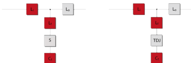
Figure 1 Filter configuration of FN3470, FN3472, FN3480 and FN3482
