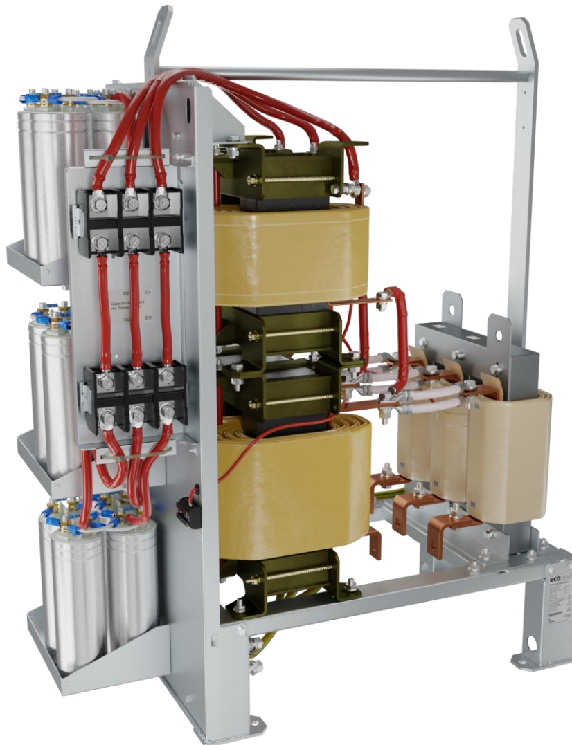
Figure 22 Design of FN3470/80/72/82 filter (Type E0XXJXX)
