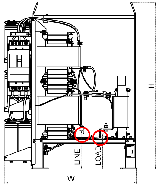
Figure 33 Location of line and load terminals for filters FN3470, FN3472, FN3480 and FN3482
