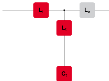
Figure 18 Schematic of FN3470, FN3472, FN3480 and FN3482 filter series
