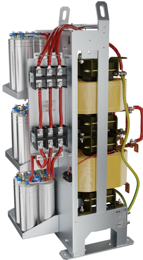
Figure 23 Design of FN3471/81/73/83 filter (Type E0XXJXX)
