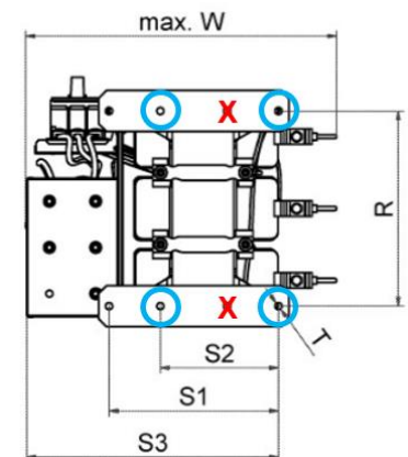
Figure 30 Permitted (blue) and forbidden (red) fixation points for filters FN3471, FN3473, FN3481 and FN3483
