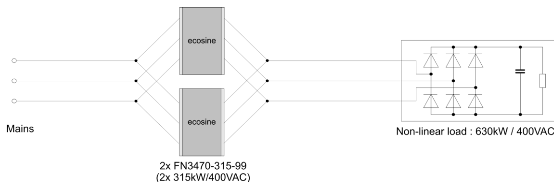
Figure 25 Application example with 2 filters in parallel for larger load
