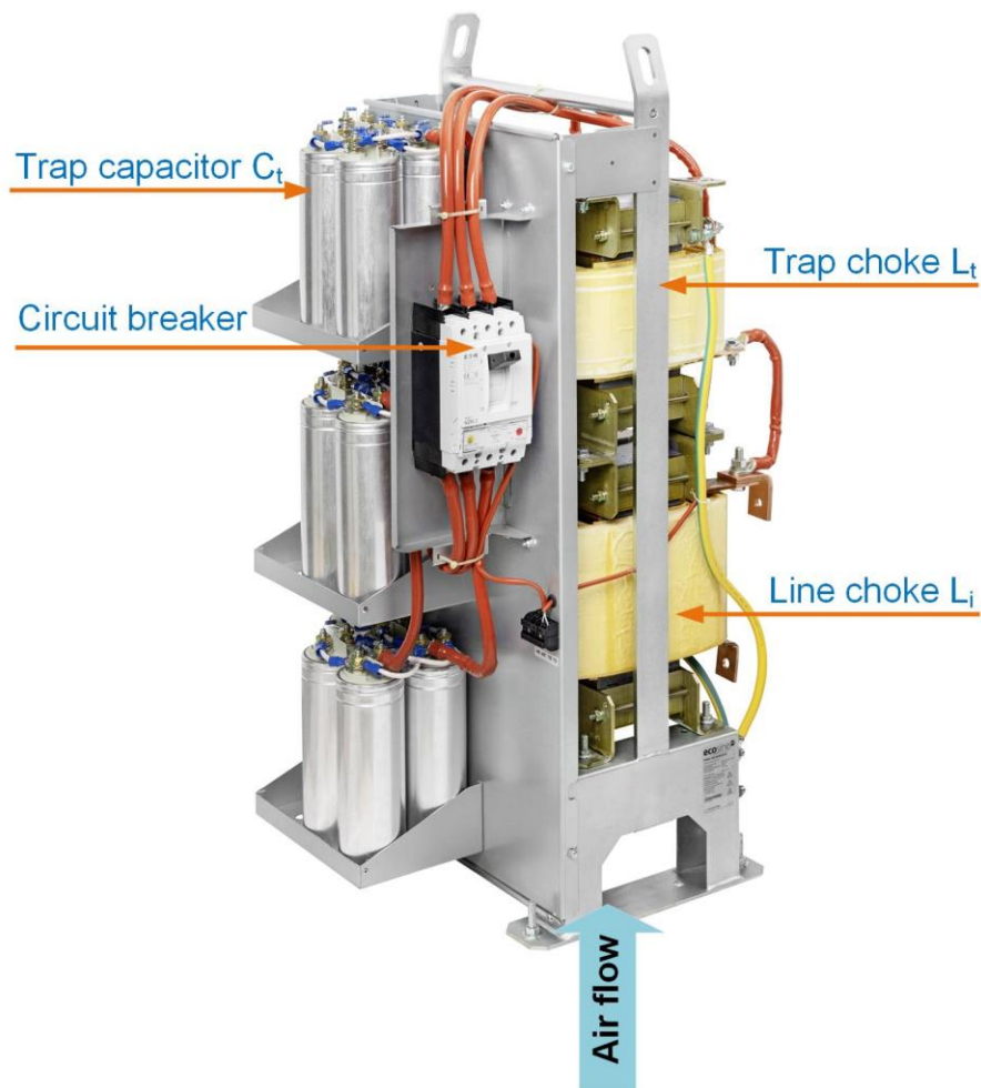
Figure 21 Design of FN3471/81/73/83 filter (Type E0XXSXX)
