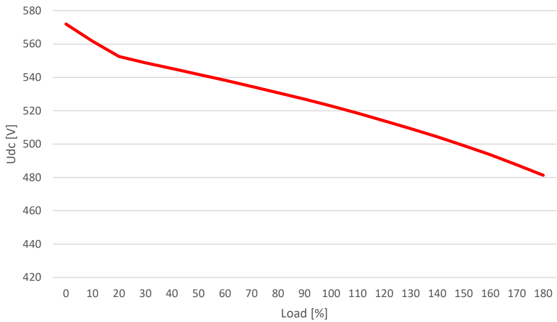
Figure 16 Drive dc-link voltage vs. load (diode rectifier front-end, with FN3471 series and drive with 4% Ldc)
