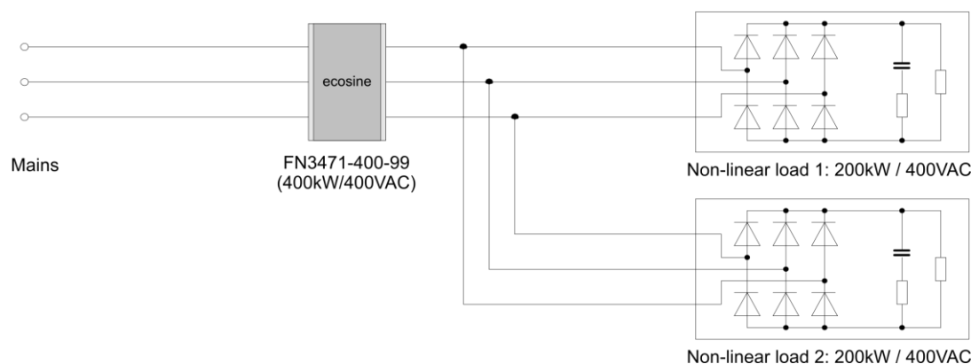
Figure 24 Application example with multiple loads per filter
