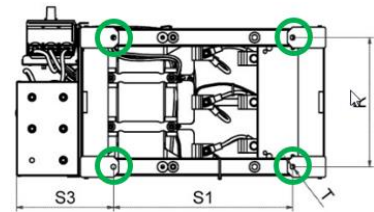
Figure 28 Fixation points for filters FN3470, FN3472, FN3480 and FN3482
