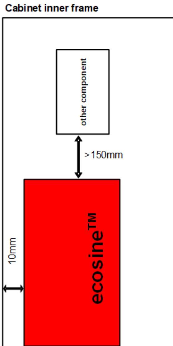
Figure 27 Clearance inside cabinet
