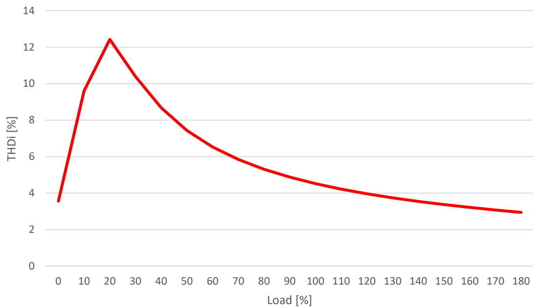
Figure 14 THDi vs. load (diode rectifier front-end)
