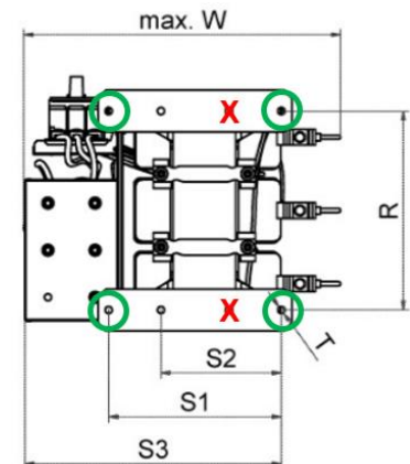
Figure 29 Preferred (green) and forbidden (red) fixation points for filters FN3471, FN3473, FN3481 and FN3483
