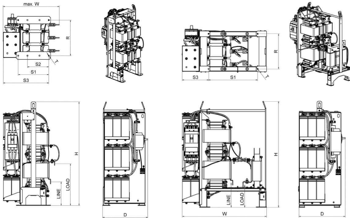
Figure 10 Mechanical data of FN3471/73/81/83 with S option (switch integrated).
