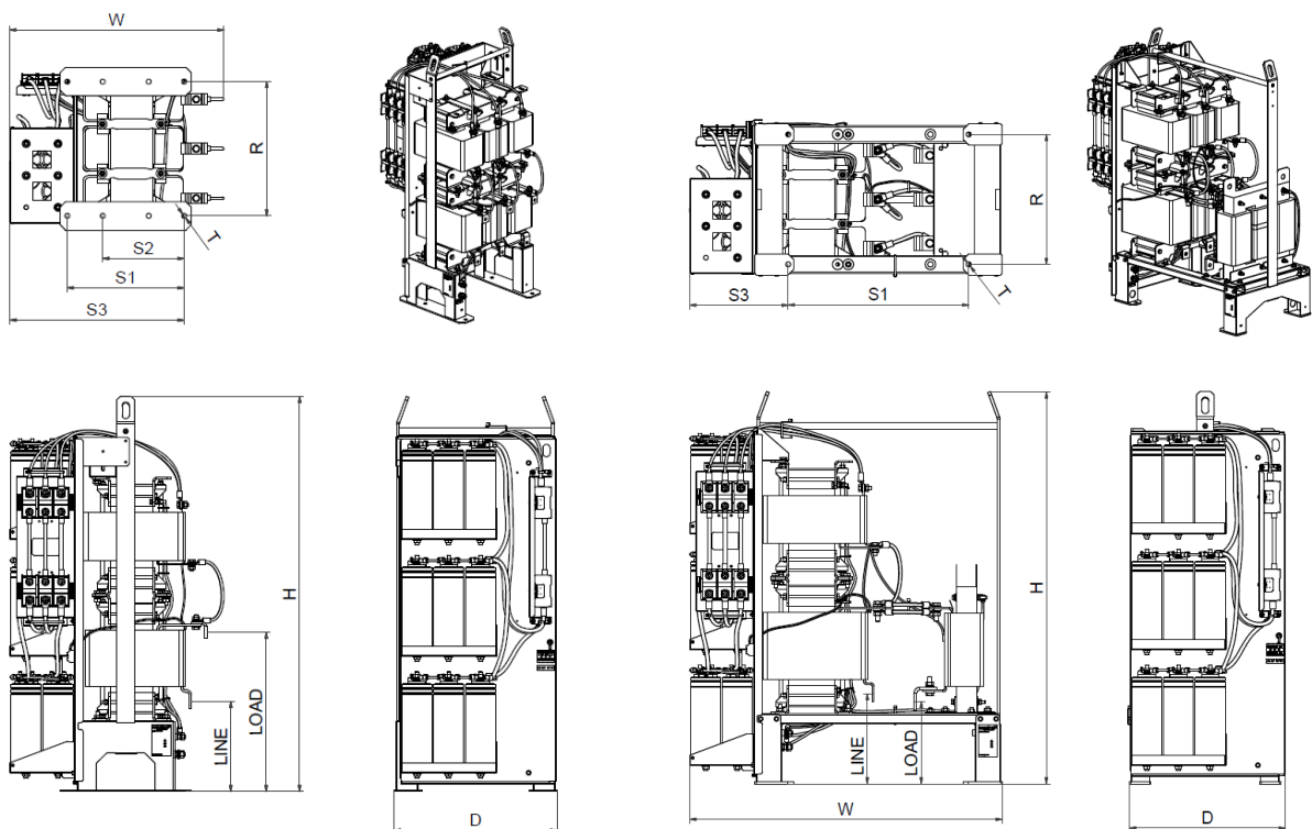
Figure 12 Mechanical data of FN3471/73/81/83 with J option (Trap Disconnect Terminals).
