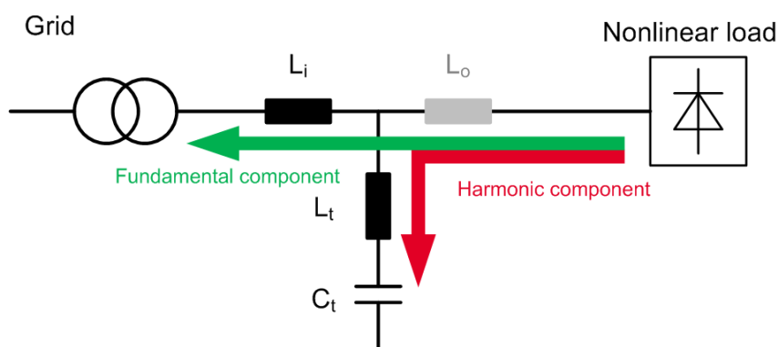
Figure 19 Working principle of Ecosine Max Passive Harmonic Filters (with load choke L_o and without)
