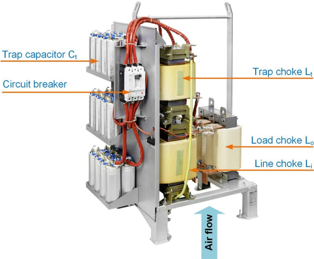
Figure 20 Design of FN3470/80/72/82 filter (Type E0XSXX)
