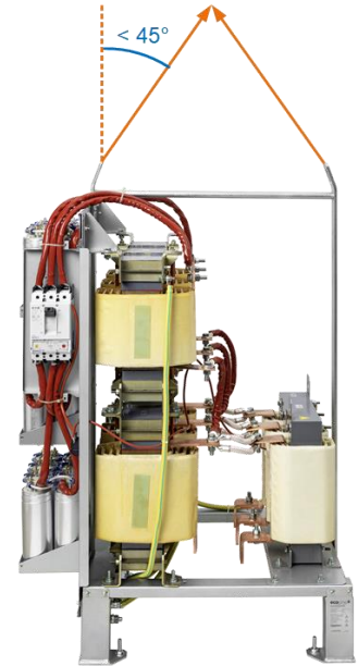
Figure 32 Maximum angle of lifting force
