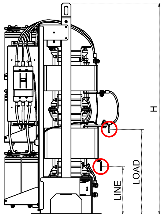
Figure 34 Location of line and load terminals for filters FN3471, FN3473, FN3481 and FN3483
