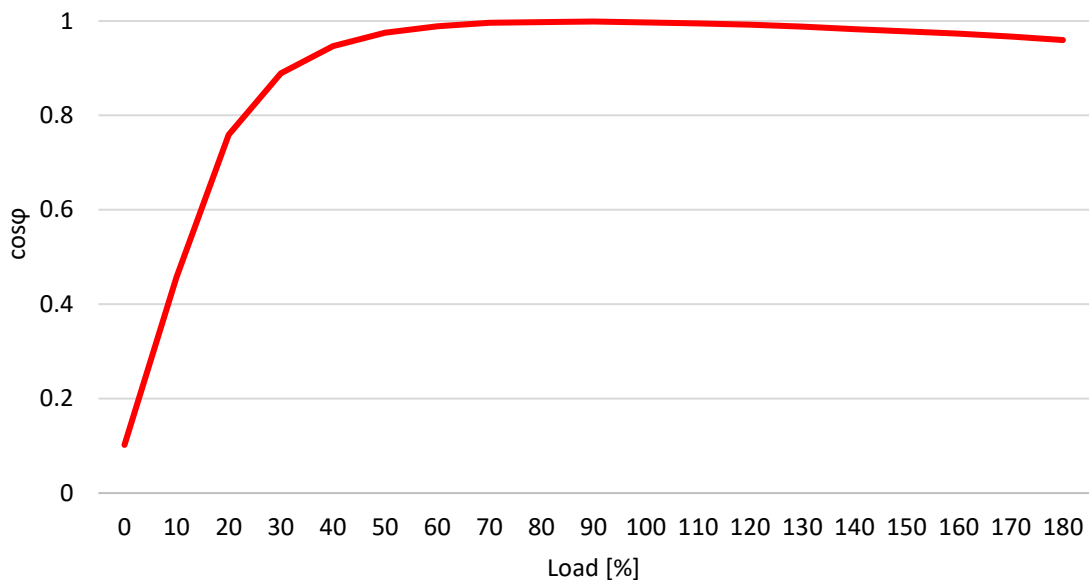
Figure 37 Power factor vs. load (diode rectifier front-end) (see section 3.13)
