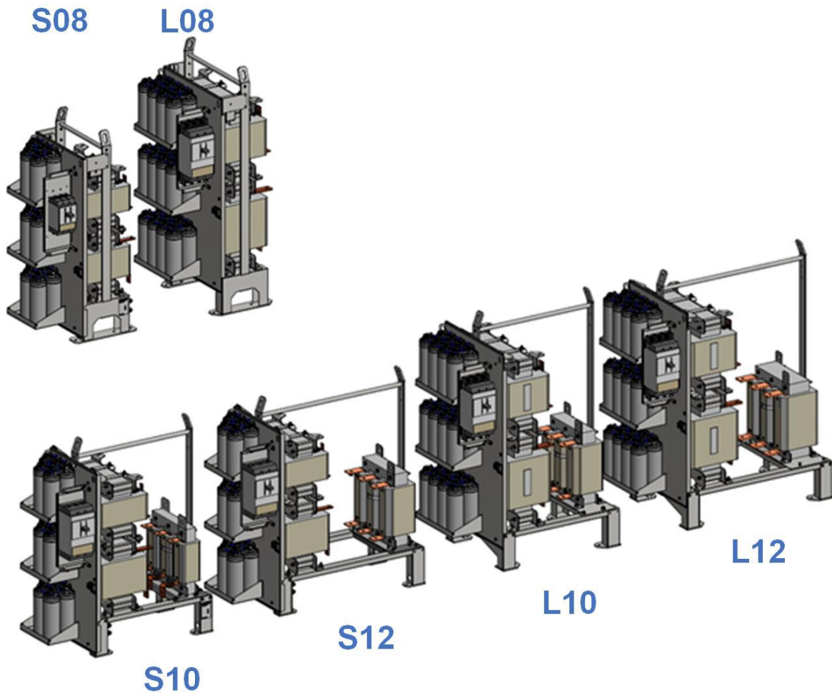
Figure 9 Overview of all Ecosine Max Passive Harmonic Filters frame sizes
