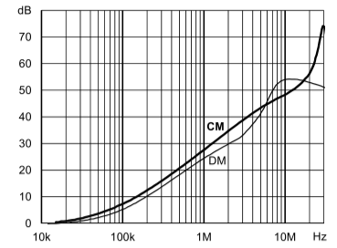
FN261/ FN9260: 6 and 10 A types
